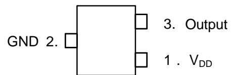
SC59
